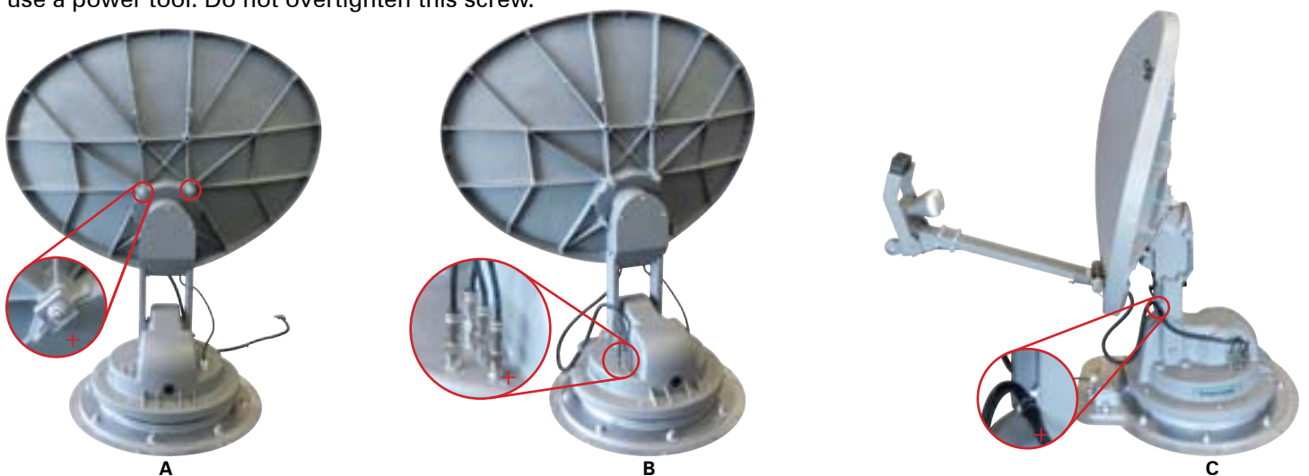
FIGURE 2. Installing reflector, LNBF, and feed arm. A, Reflector held on skew plate with clamps. B, Coax cables connected. C, P-clamp on lift arm.
